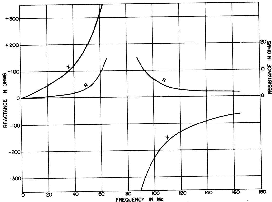
Figure 5. Generator Terminal Impedance plotted versus Frequency.
