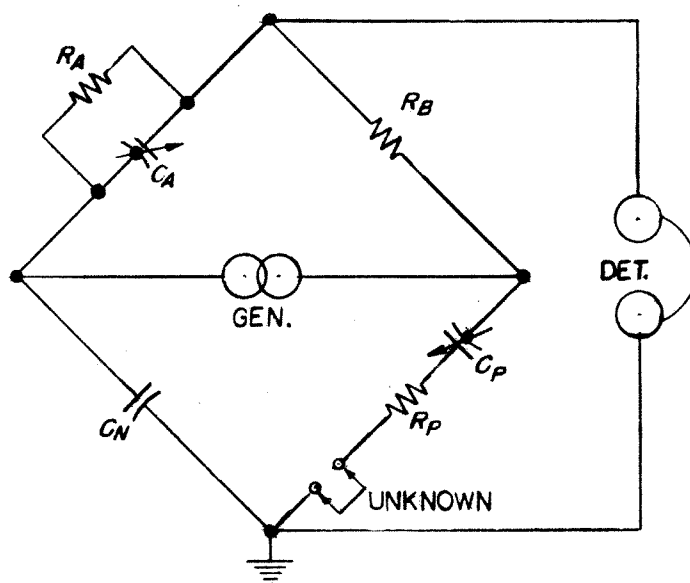
Figure 1. Basic Circuit of the Type 1601-A V-H-F Bridge.
