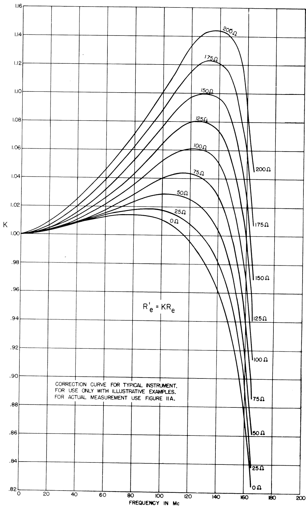
Figure 11. Correction Chart for Inductance in Resistance Capacitor.
